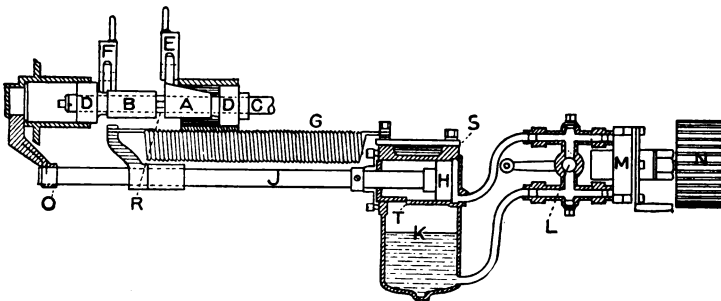
FIG. 217.—Diagram of the Cadillac Variable-Cam Oil-Governor Regulation.
